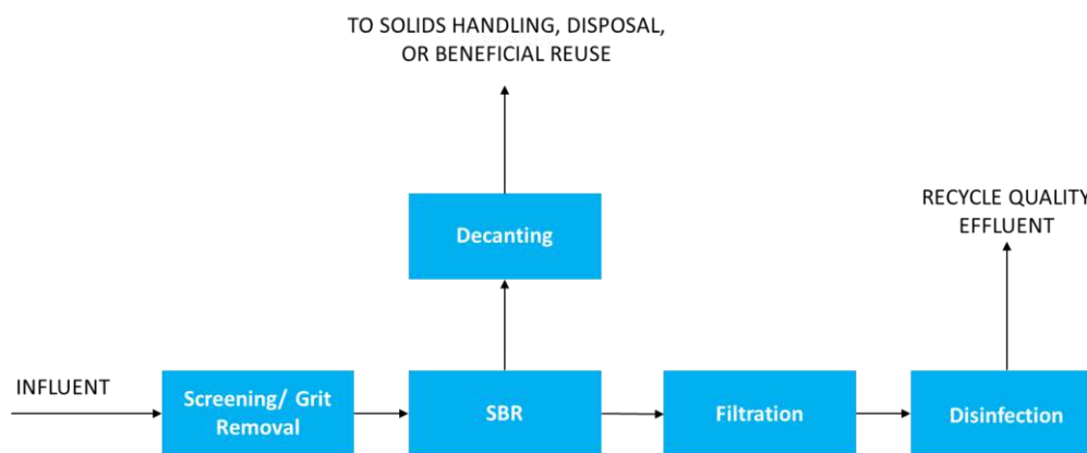
Exhibit 5.13: Process flow diagram for a typical SBR
